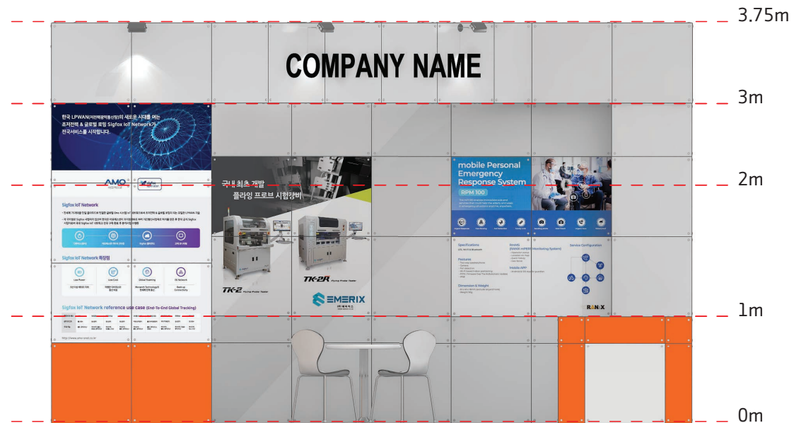
| Front view
